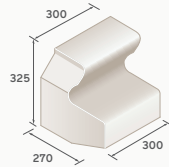
Clockwise Chevron unit
