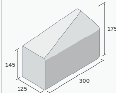
Transition to Dropper (L/H shown)
