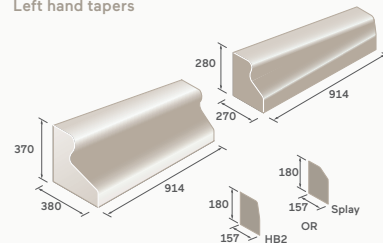
Left hand tapers
