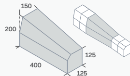
BNBN Converts Bullnose High Kerbs to Bullnose Drivestyle Kerbs
