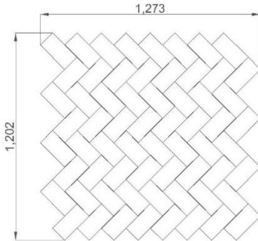
64 block cluster formation, as viewed by the machine lay operative.
