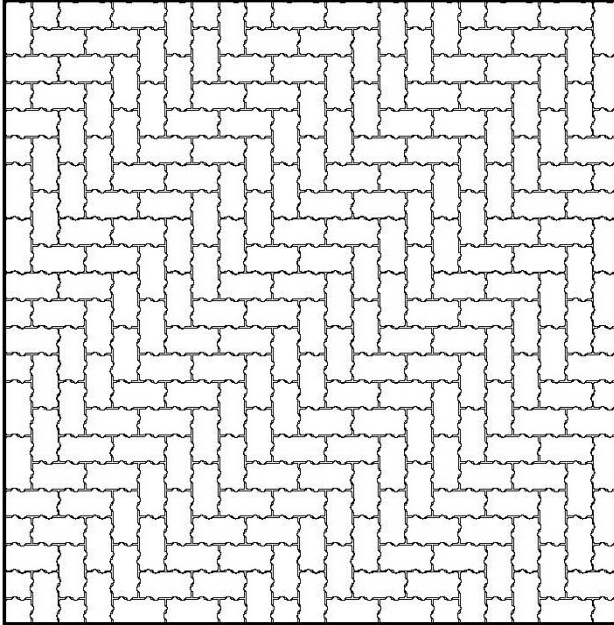
Pattern LN.05 - Double Herringbone - P & L*
