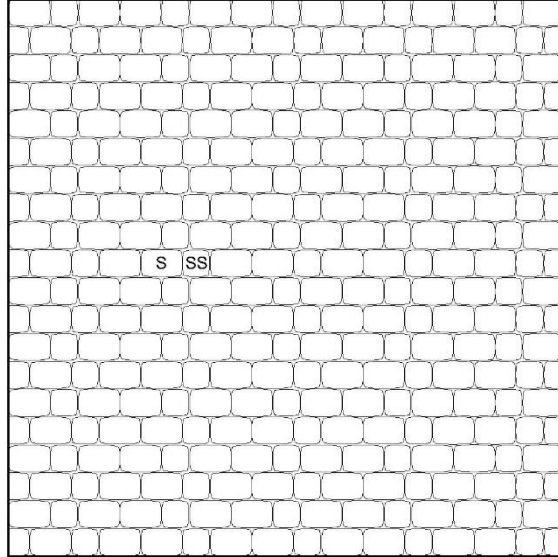
Pattern AUR.02 - Stretcher Course 1:2 - P & L*
