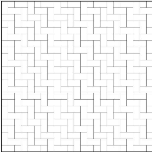
Pattern OMP.01 - Herringbone 90° - P,L & C
