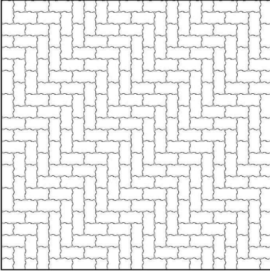
Pattern OMF.05 - Double Herringbone - P & L*
