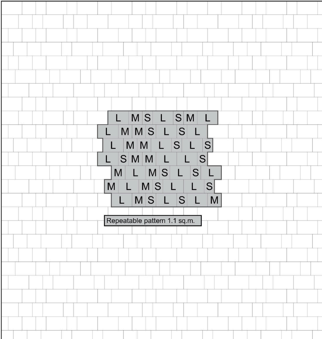
Pattern LUT.01 - Stretcher Bond - P & L*
