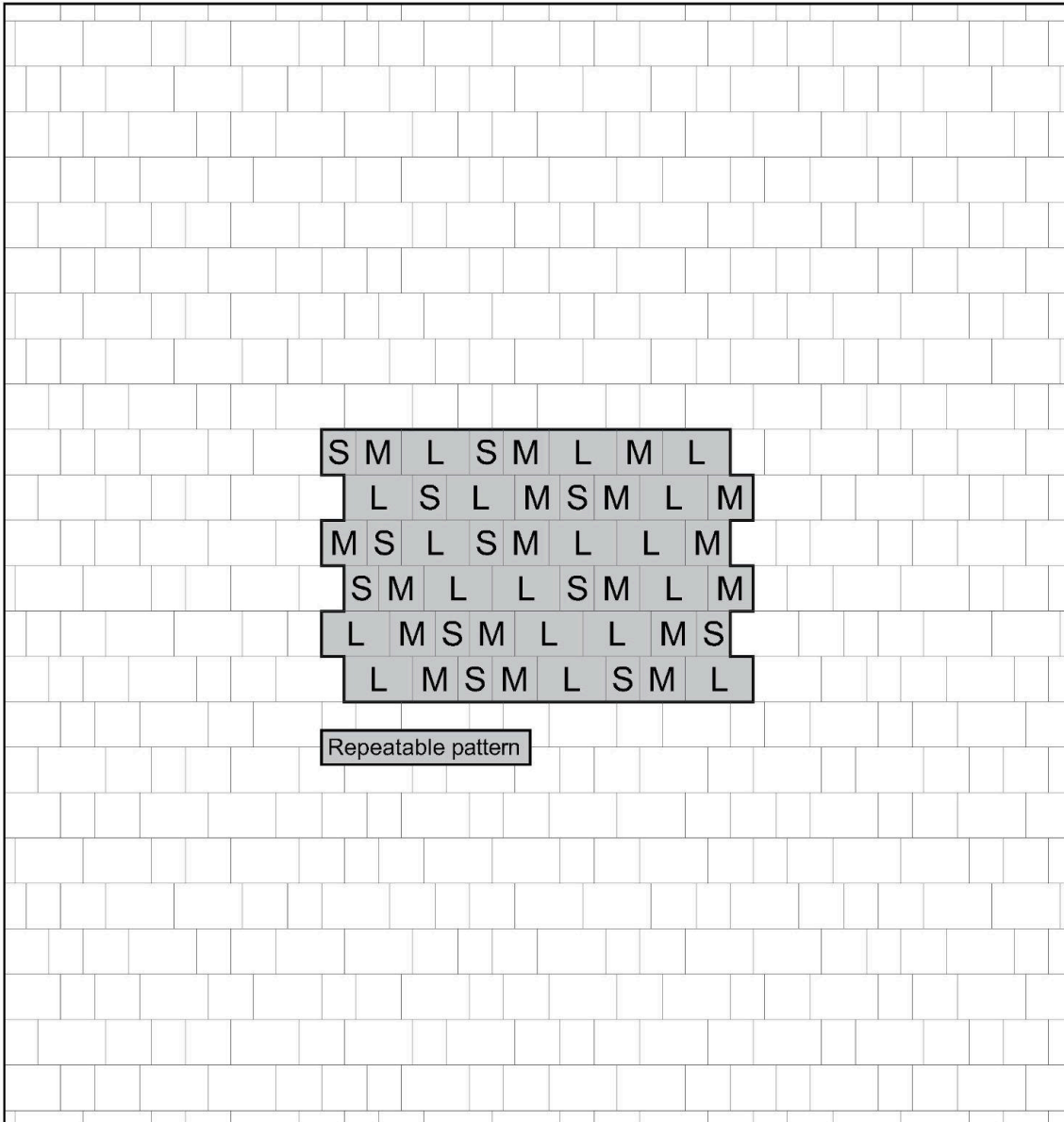
Pattern ALT.01 - Stretcher Bond - P & L*
