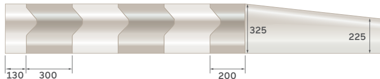
Front elevation with anti-clockwise directional indication
