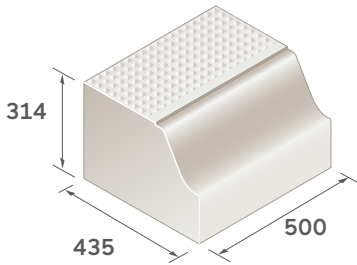
Half Kerb 160mm
