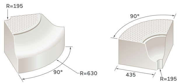
90° quadrant (external or internal)
