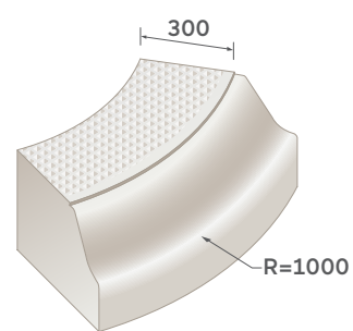
45° external quadrant
