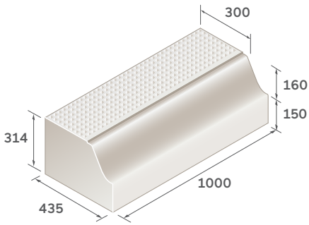
Standard Kerb 160mm
