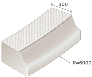
6m external radius
