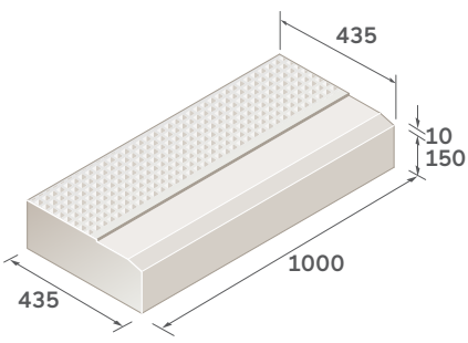
Flat Kerb
