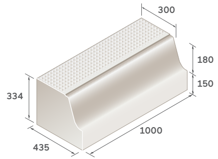
Standard Kerb 180mm
