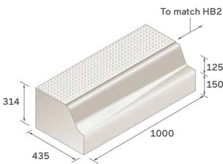
Left hand transition 160mm
