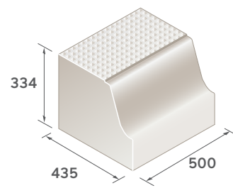
Half Kerb 180mm
