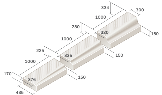
Right hand transition 180mm
