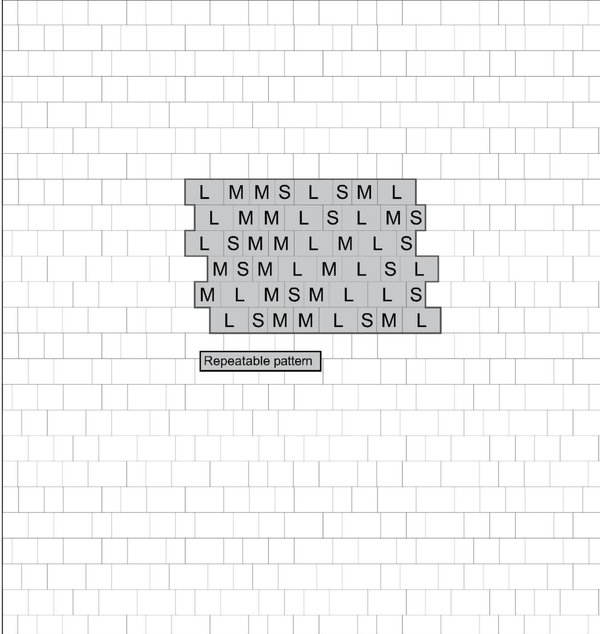
Pattern LUT.02 - Stretcher Bond - P & L*
