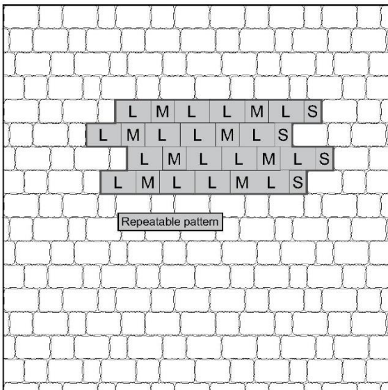
Pattern ALF.07 - 3 Size Stretcher - P & L*
