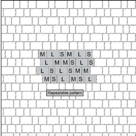
Pattern ALF.05 - 3 Size Stretcher - P & L*
